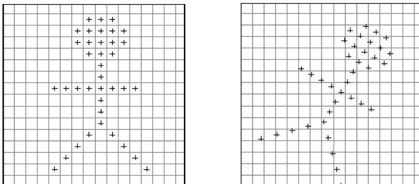
Figure 5-1: Original Pixel Center Locations (Left) and Rotated Pixel Center Locations (Right)
