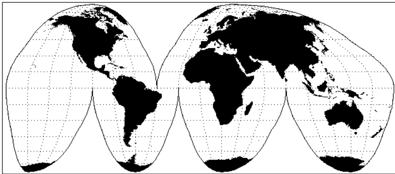
Figure 7-16: Goode's Homolosine Projection
